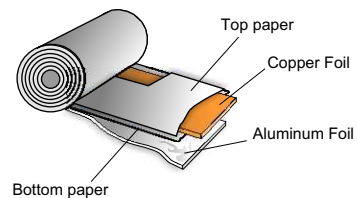
Rolled Earth Capacitor
